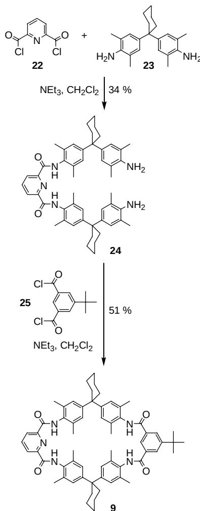
Scheme 3 Synthesis of macrocycle 9
